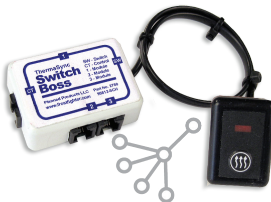
ThermaSync® Switch Boss activates several defrosters from a single switch.
